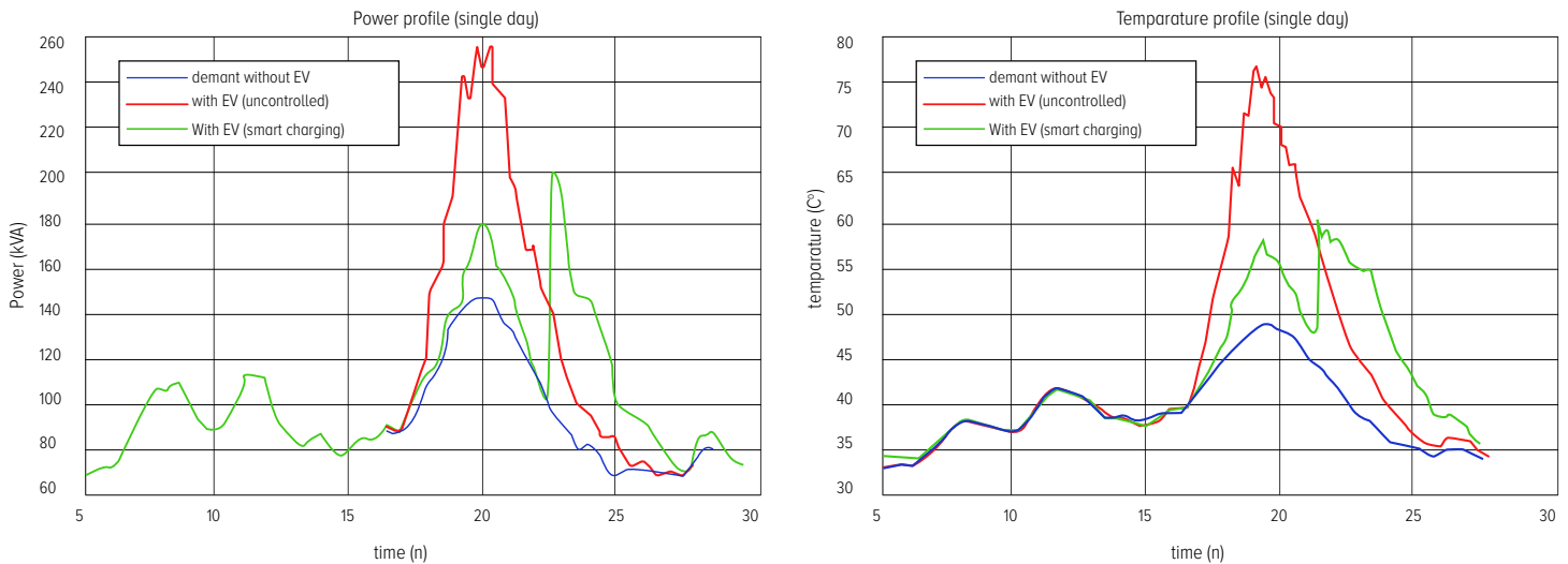
Figure 3: Impact of EV charging on transformer loading conditions (power and temperature). Simulation with a 250 kVA transformer, 40 EV and 7.4 kVA charging points in a collective residential building
