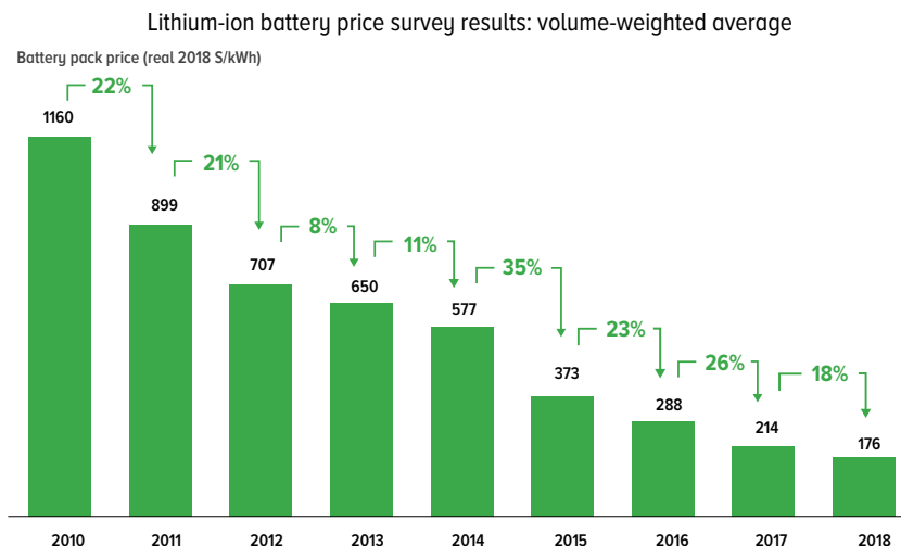
Figure 2: Evolution of battery costs (source: Bloomberg New Energy Finance)
